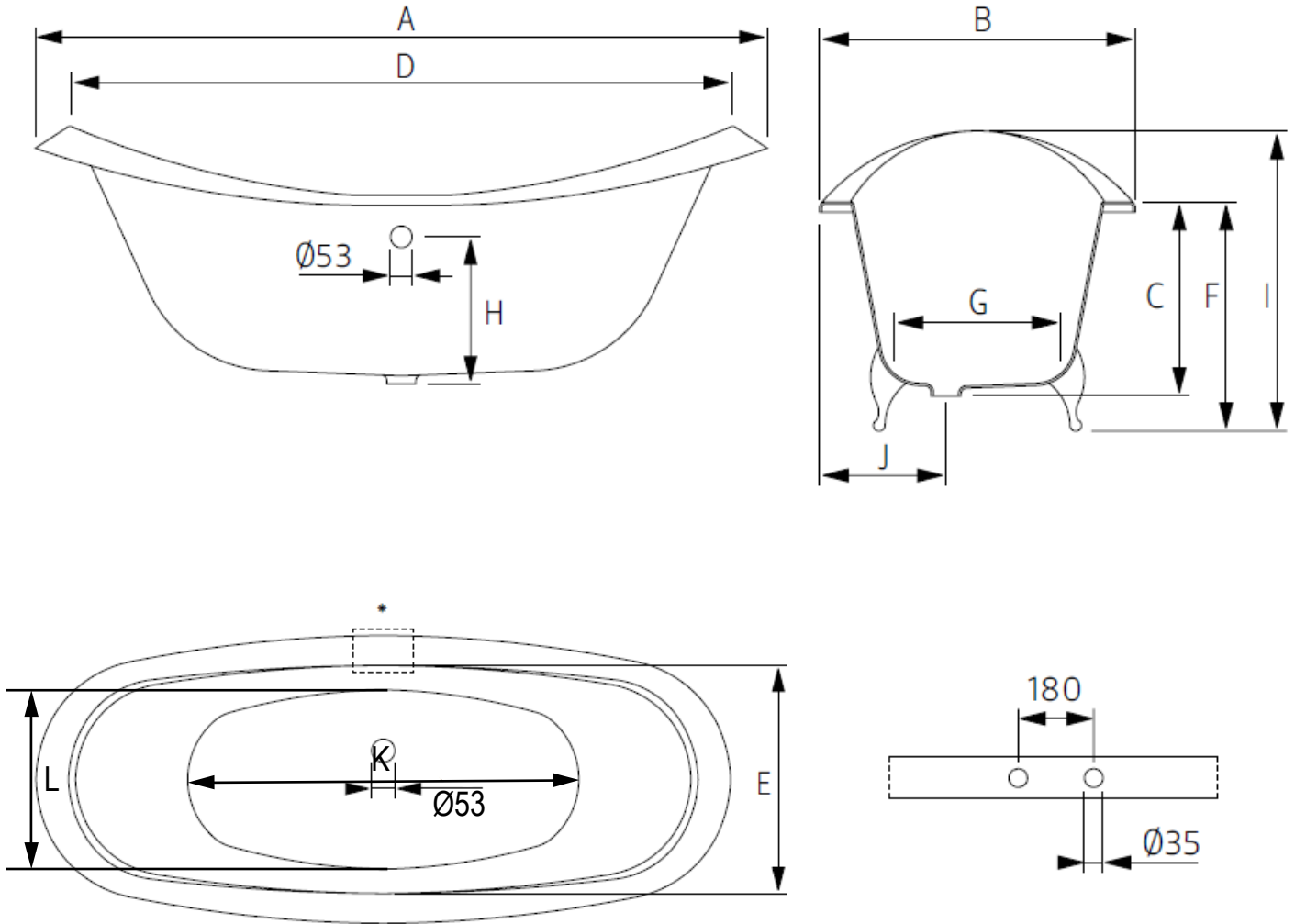
DIMENSIONS (mm)
